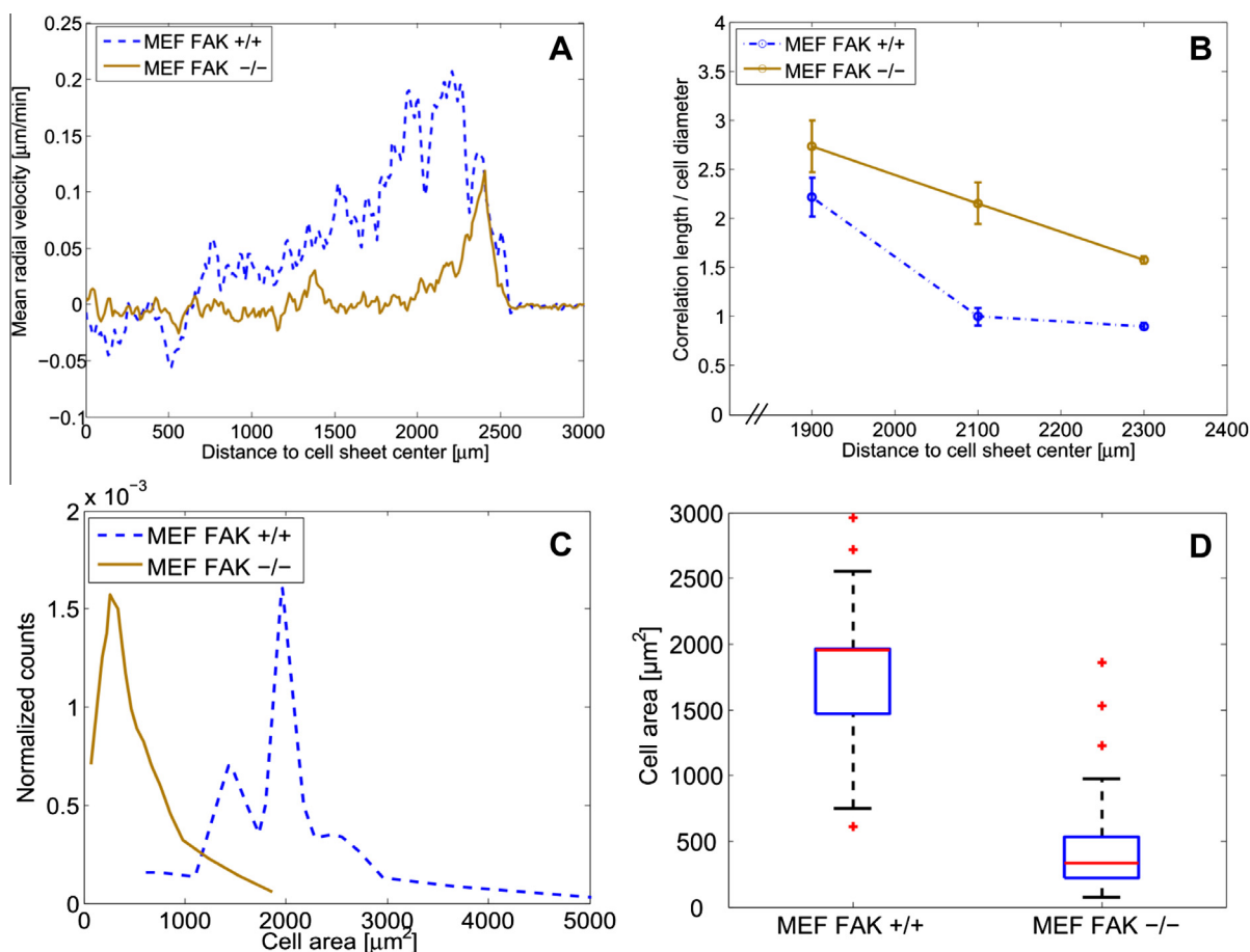
Fig. 4. Data computed from displacement fields of the radial section of cell colonies by MatLab particle image velocimetry. (A) Averaged radial cell speed for MEF FAK +/+ and MEF FAK -/- cells. (B) Directional correlation length as a function of distance (center → front). (C) Distribution of the different cell areas. (D) The average cell size of MEF FAK -/- cells was by a factor of four smaller compared to MEF FAK +/+ cells.
